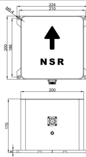
COMPASS UNIT
